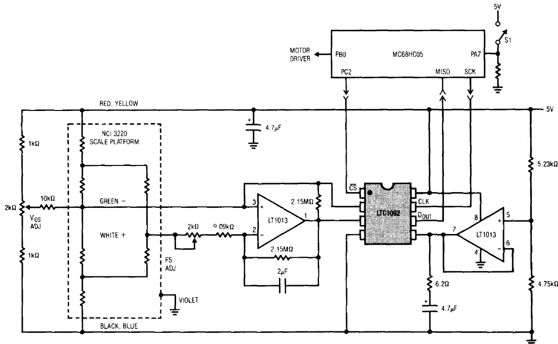
Figure 2. This Circuit Determines Small Weight Changes, Permitting Accurate Filling. Using the Appropriate Transducer, Containers may Range from Perfume Bottles to Railroad Cars.
